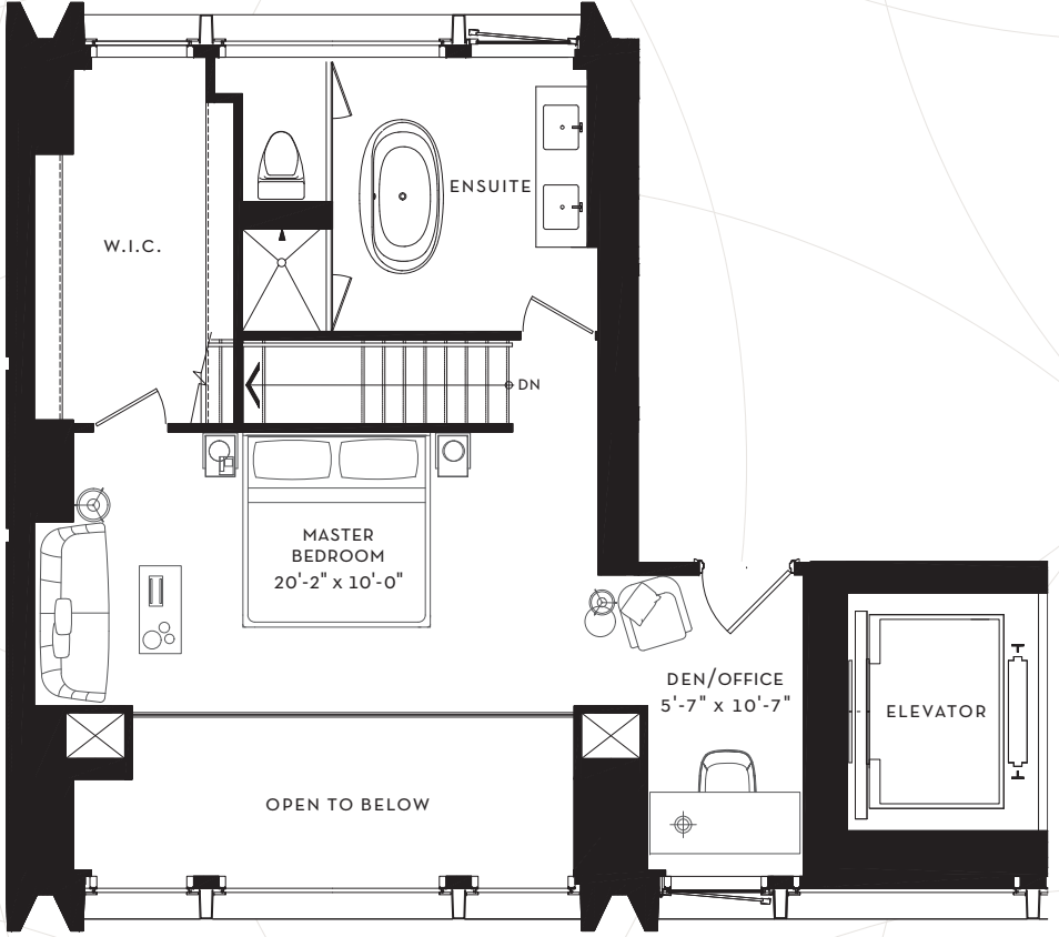
DUPLEX-LEVEL 2
